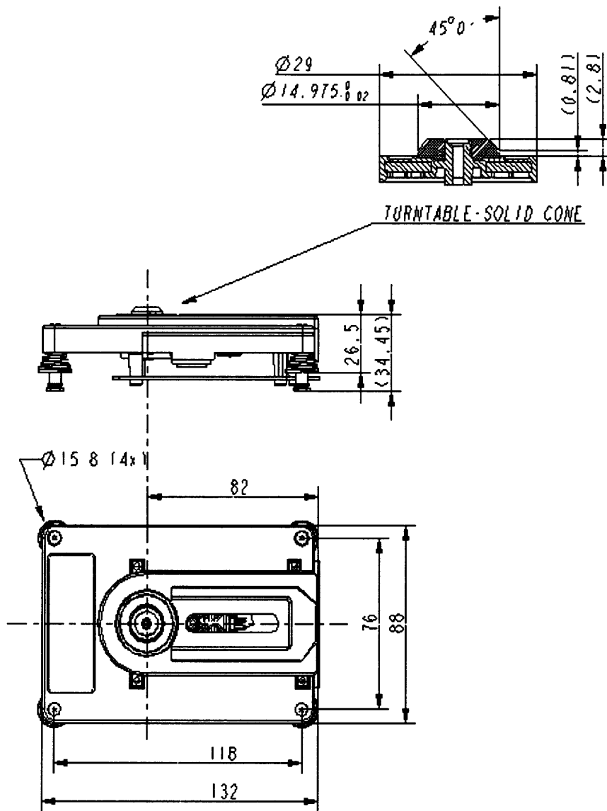
Fig 8: Dimension sketch
